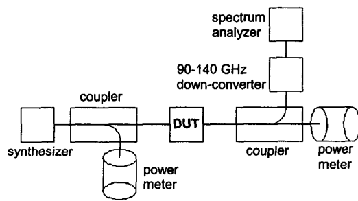
Fig. 5. Diagram of the test setup.
