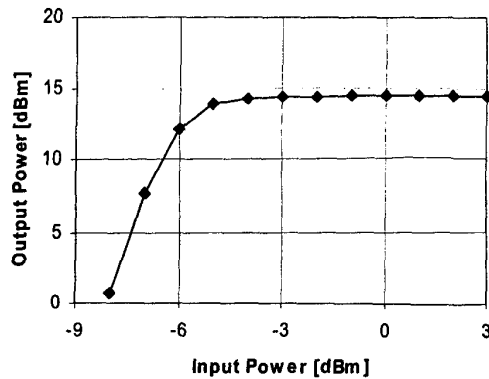
Fig. 8. Output power versus input power at 96 GHz. The gain control voltage was fixed at -1V for maximum gain.
